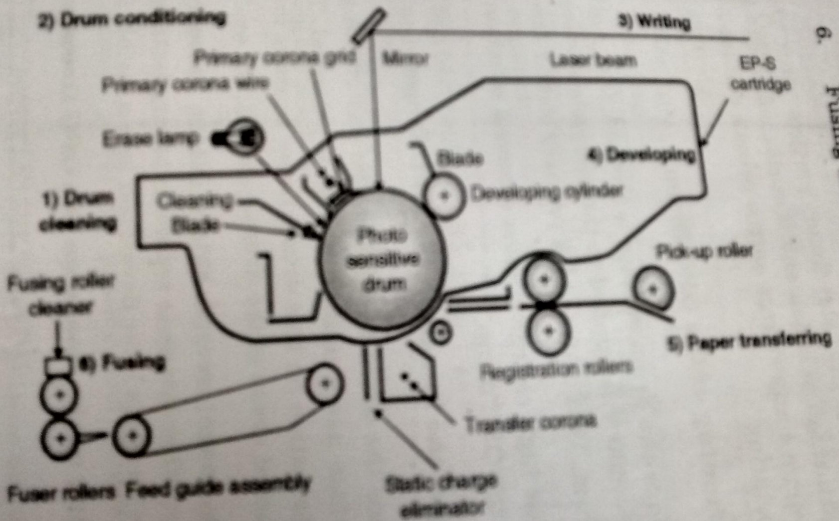
Fig. 4.24 : An image formation process in laser printer
